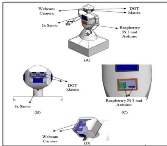
FIGURE 1. (A-D). Component design on a humanoid robot.
