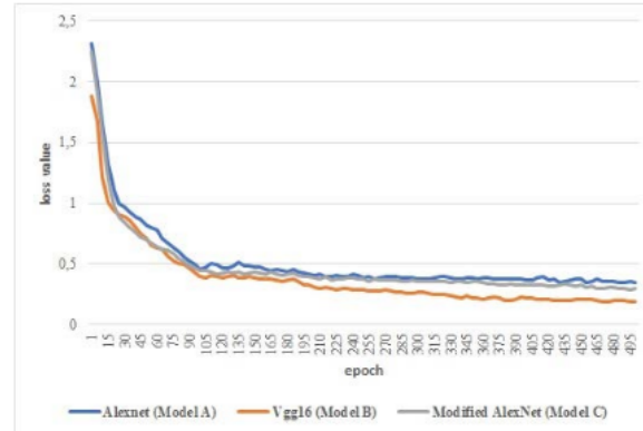
FIGURE 9. Training loss in emotion recognition.
