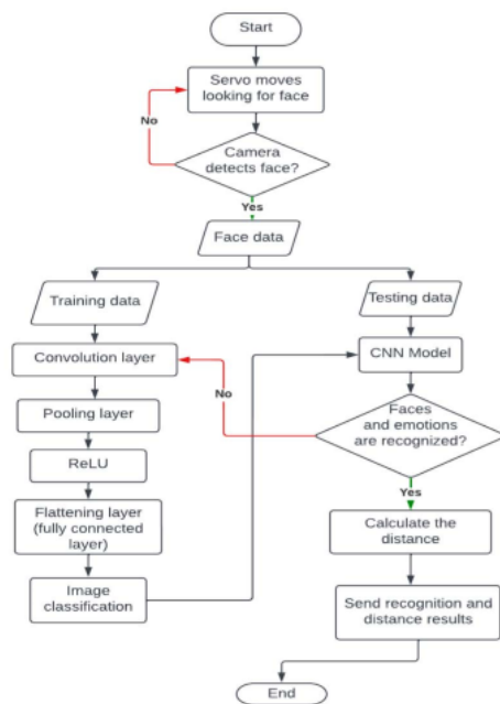
FIGURE 2. Design of the recognition system.
