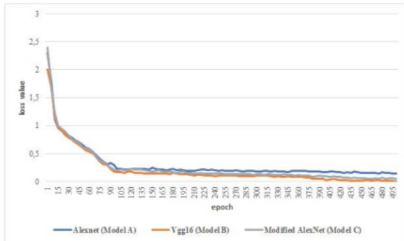
FIGURE 7. Training loss in face recognition.
