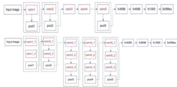
FIGURE 3. AlexNet architecture (above) and VGG16 (below) [34].
