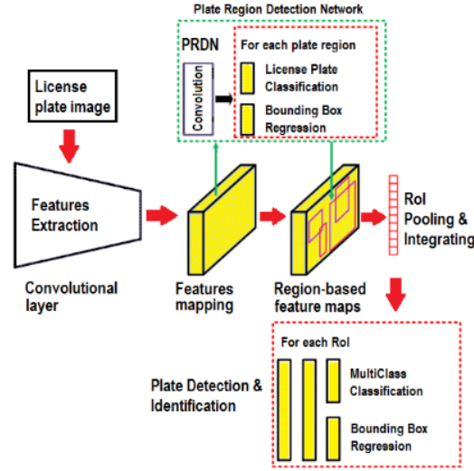
Fig. 1. Conceptual Model.
