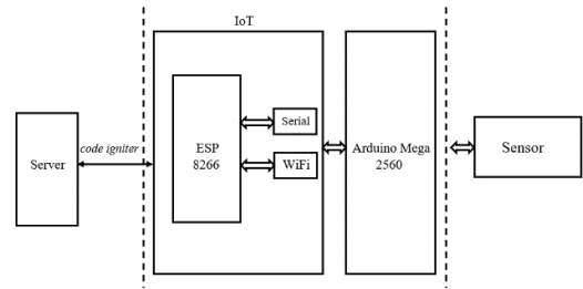
Figure 9. IoT Architecture
