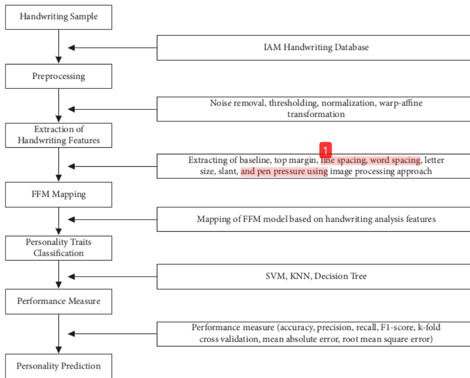
FIGURE 1: Proposed framework.
