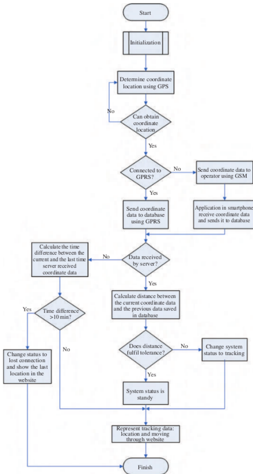
Figure 21.3 Flowchart tracking system using GPS
