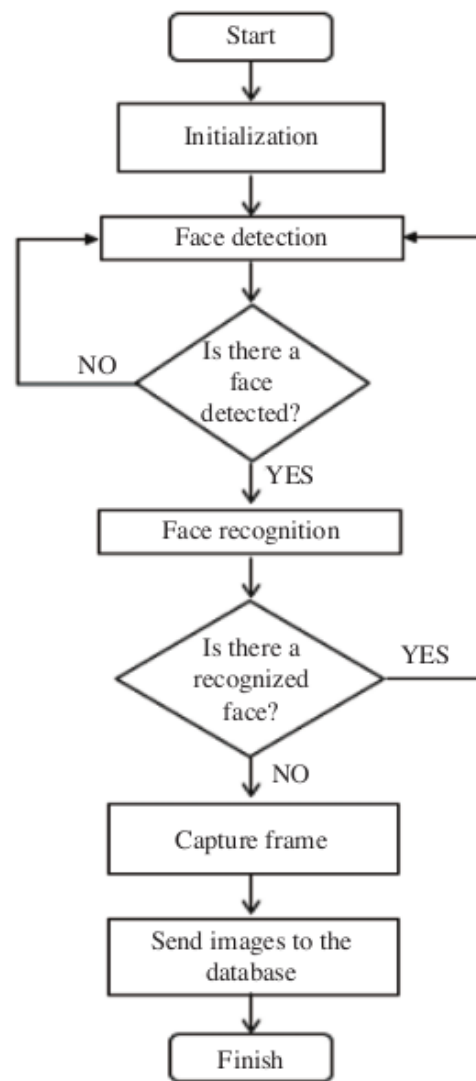
Figure 21.1 Flowchart for face recognition system
