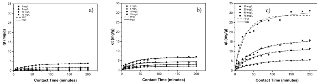
Fig. 8. Effect of adsorption time of methylene blue on Zn/Al LDH a), biochar b), and composite c).
