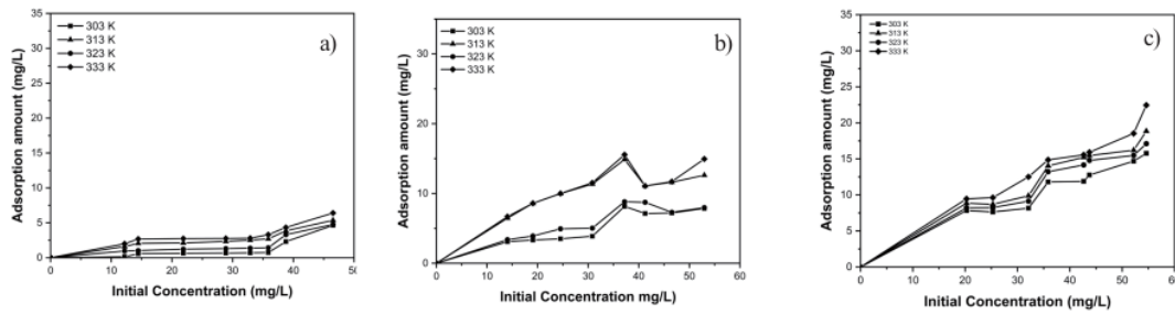
Fig. 9. The effect of initial concentration of methylene blue and temperature adsorption on Zn/Al LDH a), biochar b), and composite c)
