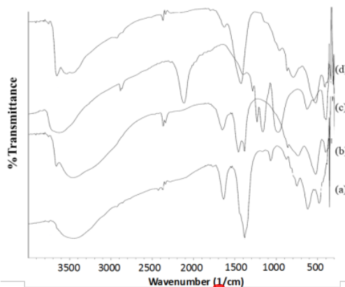
Figure 4. FTIR spectrum of Ca/Al LDH (a), calcination of Ca/Al LDH at 800 °C (b), polyoxometalate \text{K}_4[\alpha\text{-SiW}_{12}\text{O}_{40}]\cdot n\text{H}_2\text{O} (c), and intercalated Ca/Al LDH with \text{K}_4[\alpha\text{-SiW}_{12}\text{O}_{40}]\cdot n\text{H}_2\text{O} (d)
