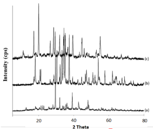
Figure 2. XRD powder pattern of Ca/Al LDH (a), calcination of Ca/Al LDH at 800 °C (b), and intercalated Ca/Al LDH with \text{K}_4[\alpha\text{-SiW}_{12}\text{O}_{40}]\cdot n\text{H}_2\text{O} (c)
