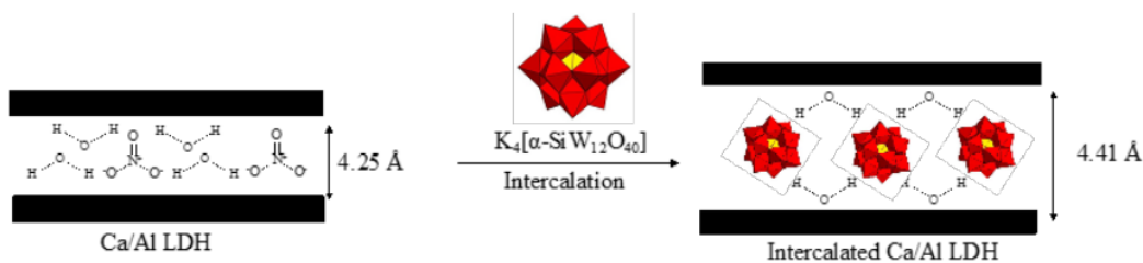
Figure 3. Illustration of intercalation Ca/Al LDH with [\alpha\text{-SiW}_{12}\text{O}_{40}]^{4-}
