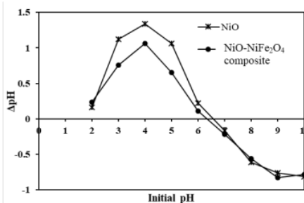
Fig. 6. pHPzc values of NiO and NiO-NiFe 2 O 4 composite.
