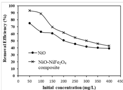
Fig. 8. Photocatalytic degradation of Congo red dye by variation of initial concentration.
