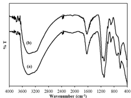
Fig. 2. FTIR spectra of (a) NiO and (b) NiO-NiFe 2 O 4 composite.
