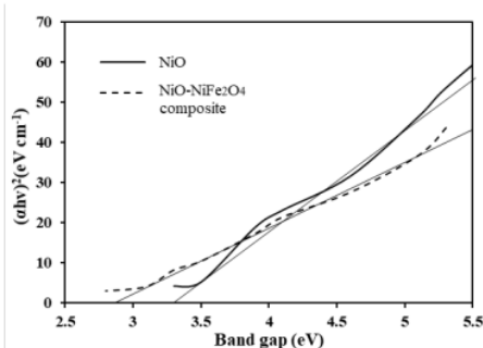
Fig. 5. Band gaps of NiO and NiO-NiFe 2 O 4 composite.
