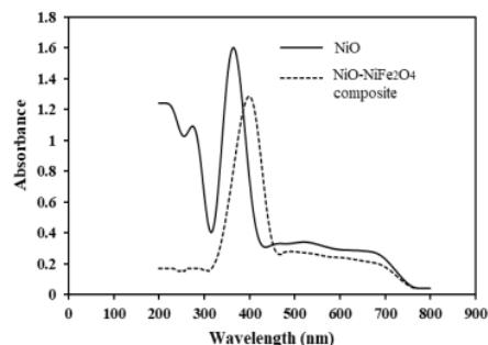
Fig. 4. Spectra UV-Vis DRS of NiO and NiO-NiFe 2 O 4 composite.
