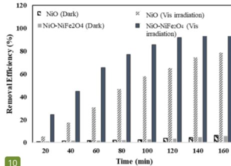
Fig. 9. Photocatalytic degradation of Congo red dye by variation of irradiation time.
