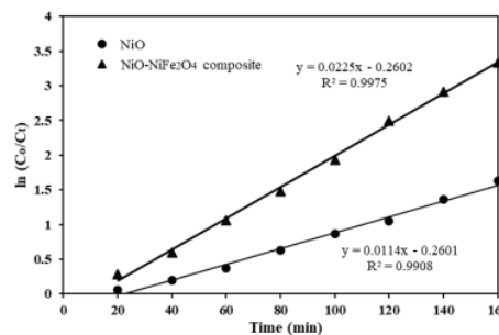
Fig. 10. Pseudo-first-order kinetics for photocatalytic degradation.
