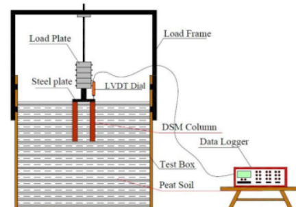
Fig. 6 DSM modeling scheme with 3.75 cm diameter with 4 columns
