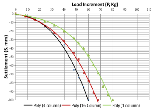
Fig. 10 Graph of load increment versus settlement for each variation (DSM with clay + RHA)
