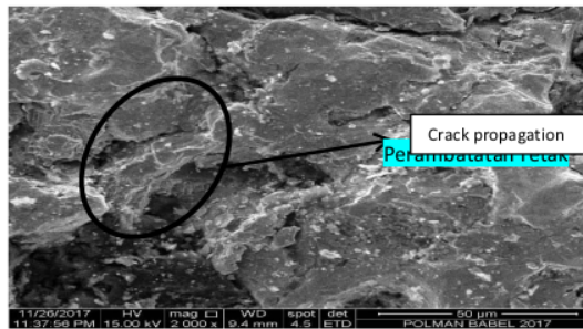
Figure 11. Scanning electron microscope of gray cast iron after normalizing 90 minutes 2000x magnification
