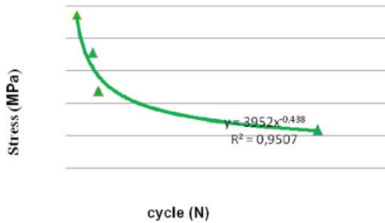
Figure 4.S-N curve Fatigue Testing Specimens With 60 min Normalizing
