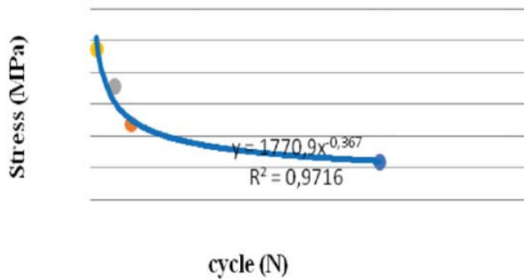
Figure 5.S-N curve Fatigue Testing Specimens With 90 min Normalizing
