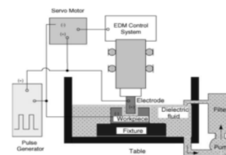
Figure 1. Schematic sinking EDM process (Lin et al. 2002)
