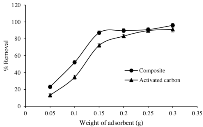
Figure 7. The effect of adsorbent weight on the adsorption of methyl red using activated carbon and \text{MnFe}_2\text{O}_4 -activated carbon composite
