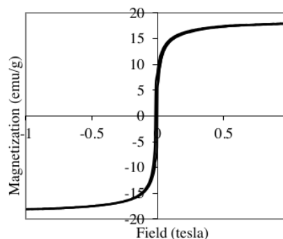
Figure 4. The Curve of magnetization of MnFe 2 O 4 -activated carbon composite
