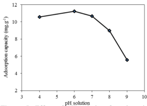
Figure 5. Effect of pH solution for adsorption capacity of phenol onto composite
