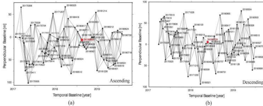
Figure 3. Perpendicular and temporal baseline networks to derive interferometric pairs. Red and black dots denote a supermaster and SAR images with the format of acquisition date [yyyymmdd], and gray lines indicate the interferogram pairs
