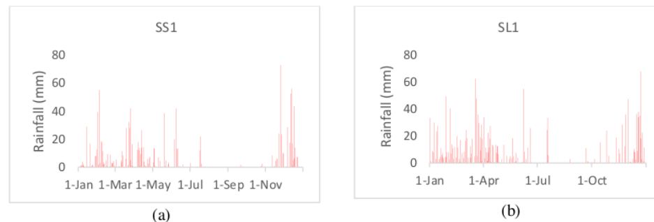
Figure 1. Time series of daily rainfall at (a) SS1 and (b) SL1
