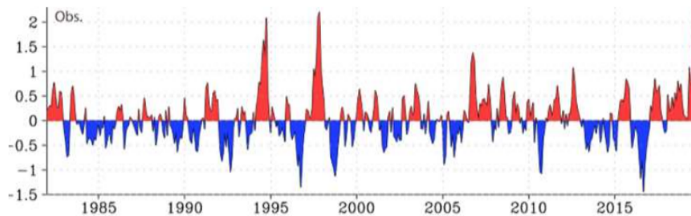
Figure 2. Graphic of Dipole Mode Index [18]
