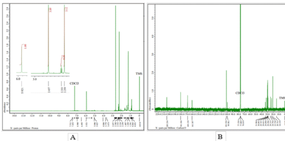
24 Figure 3. The ^1\text{H} -NMR (A) and ^{13}\text{C} -NMR (B) spectra of compound 1 ( ^1\text{H} -500 MHz; ^{13}\text{C} -125 MHz in \text{CDCl}_3 )
