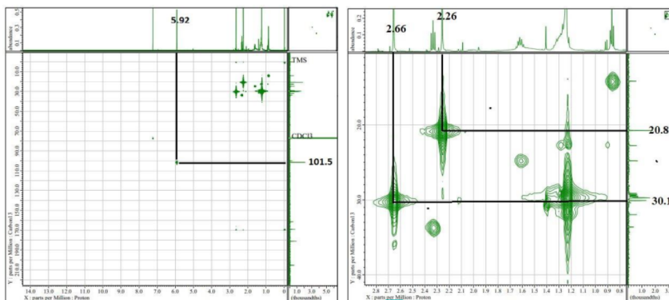
52 Figure 4. The HMBC spectra of compound 1
