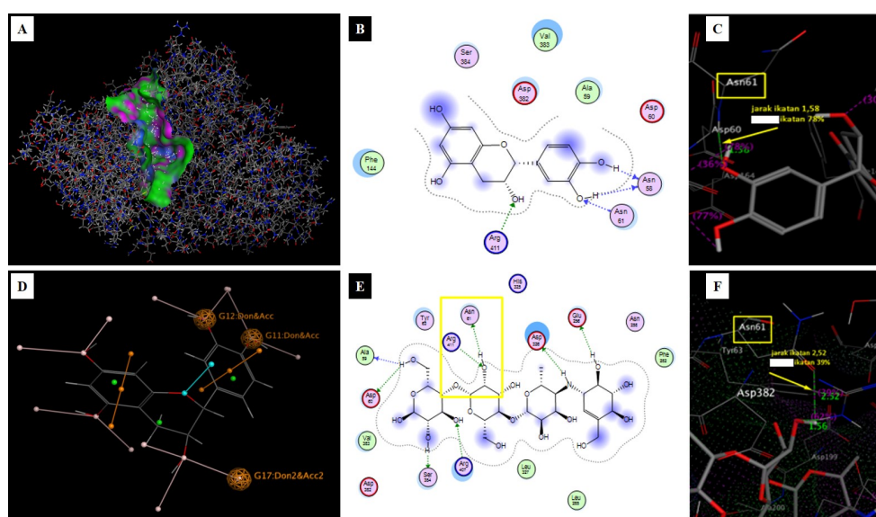
Fig. 4: Molecular Docking of Catechin with \alpha -Glucosidase
