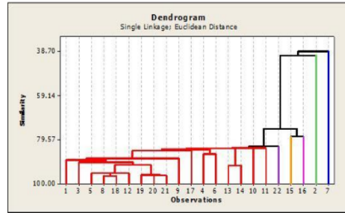
Gambar 4 Dendrogram Single Linkage
