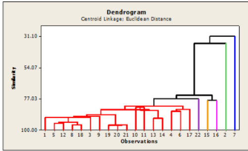
Gambar 5 Dendrogram Centroid Linkage
