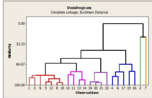
Gambar 6 Dendrogram Complete Linkage
