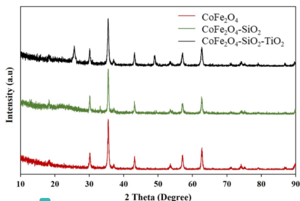
Figure 1. XRD spectra of (a) \text{CoFe}_2\text{O}_4 (b) \text{CoFe}_2\text{O}_4\text{-SiO}_2 and (c) \text{CoFe}_2\text{O}_4\text{-SiO}_2\text{-TiO}_2
