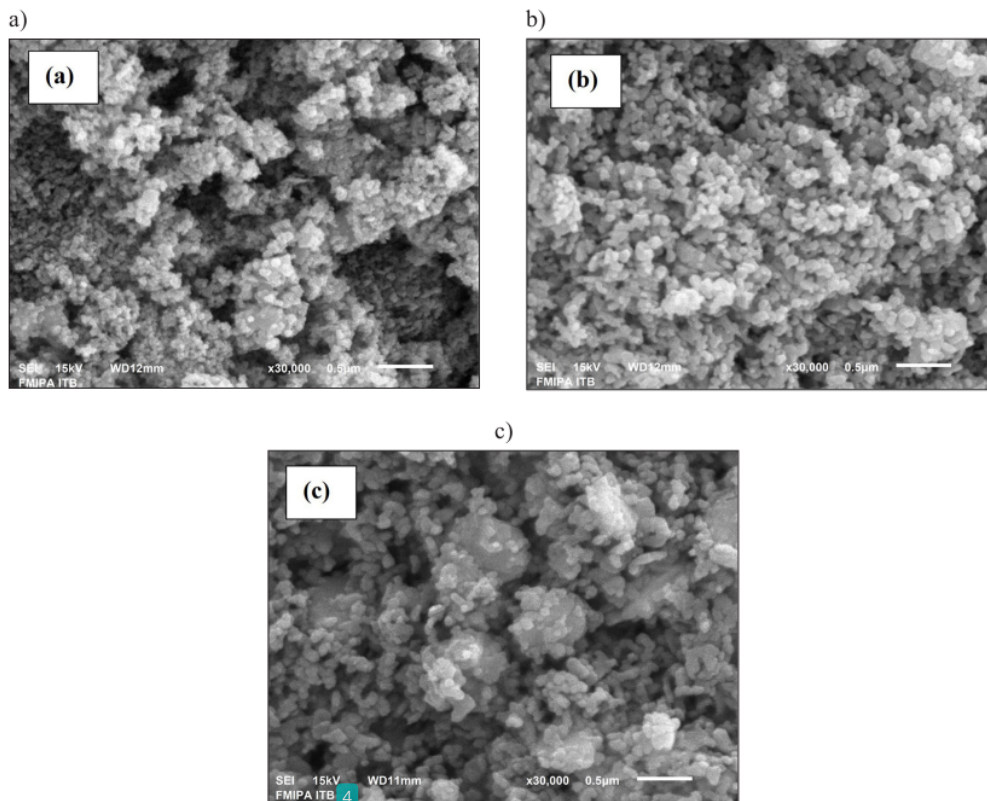
Figure 3. Morphology of (a) \text{CoFe}_2\text{O}_4 (b) \text{CoFe}_2\text{O}_4\text{-SiO}_2 and (c) \text{CoFe}_2\text{O}_4\text{-SiO}_2\text{-TiO}_2
