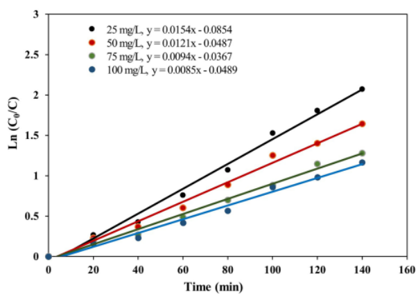
Figure 9. Kinetic photocatalytic degradation of MO by \text{CoFe}_2\text{O}_4\text{-SiO}_2\text{-TiO}_2
