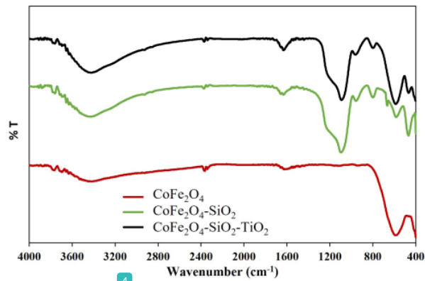
Figure 2. FTIR spectra (a) \text{CoFe}_2\text{O}_4 (b) \text{CoFe}_2\text{O}_4\text{-SiO}_2 and (c) \text{CoFe}_2\text{O}_4\text{-SiO}_2\text{-TiO}_2
