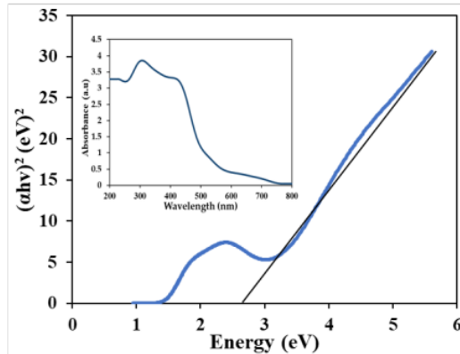
Figure 7. Wood-Tauc plot for \text{Fe}_3\text{O}_4/\text{SiO}_2/\text{NiO}
