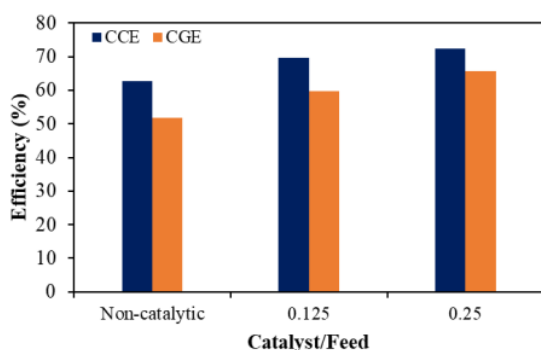
Figure 9: Effect of Catalyst on Gasification Efficiency
