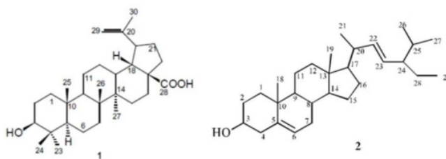
Fig. 3: Structure compounds betulinic acid (1) and stigmasterol (2)
