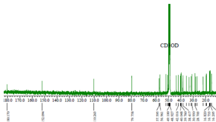
Fig. 2: ^{13}\text{C} NMR betulinic acid (1)
