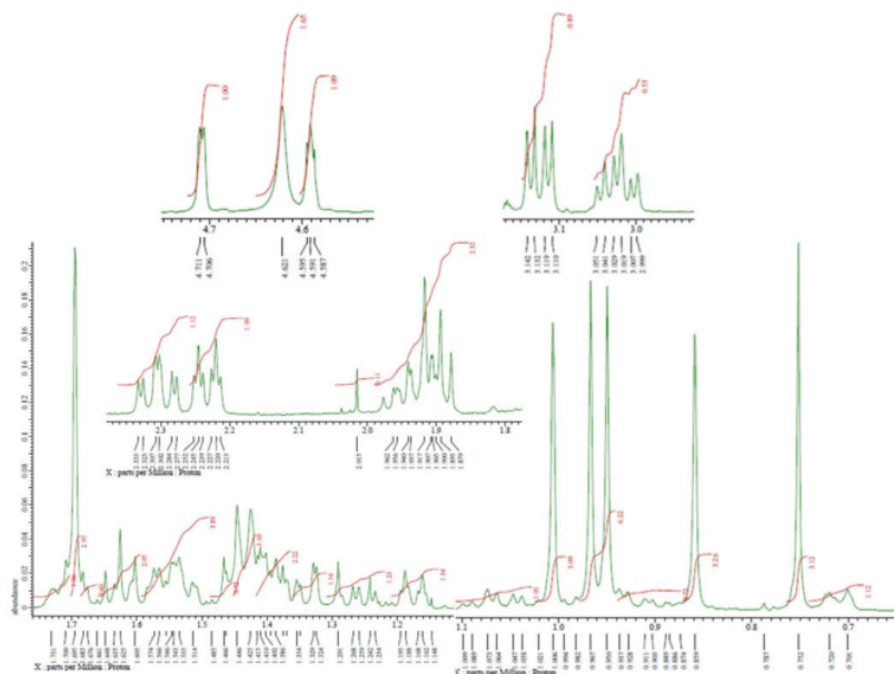
Fig. 1: ^1H NMR Betulinic acid (1)
