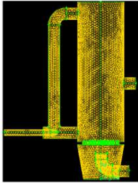
Gambar 2. Meshing Reaktor
