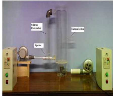
Gambar 4. Experimental Set Up
