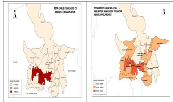
Figure 1. (a) The map of Filariasis Cases in Banyuasin, South Sumatera ; (b) Filariasis vulnerability zone area in Banyuasin, South Sumatera
