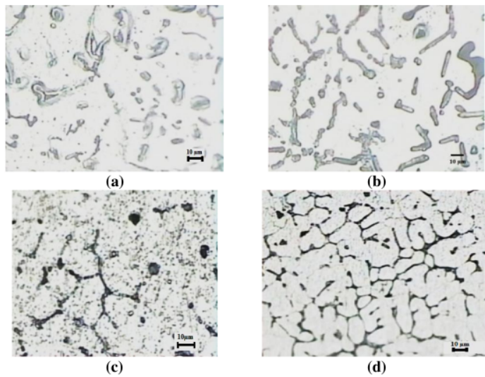
Fig. 8. Microstructure of Al-3.38%Zn alloys reinforced alumina and fly ash; (a) Alumina 8 wt% Fly Ash 0 wt% , (b) Alumina 8 wt% Fly Ash 4 wt% , (c) Alumina 8 wt% , Fly Ash 8wt% and (d) Alumina 8 wt% , Fly Ash 12 wt%.
