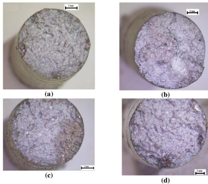
Fig. 9. Macrostructure fractography of Al-3.38%Zn alloys reinforced alumina and fly ash; (a) Alumina 8 wt% Fly Ash 0 wt% , (b) Alumina 8 wt% Fly Ash 4 wt% , (c) Alumina 8 wt% , Fly Ash 8wt% and (d) Alumina 8 wt% , Fly Ash 12 wt%
