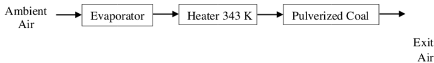
Figure 5. Research Pattern-2 for upgrading coal
