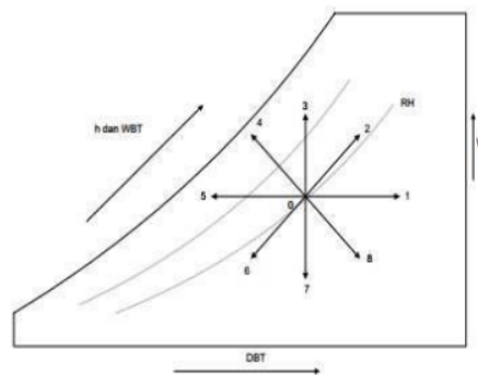
Figure 2. Psychrometric Chart
