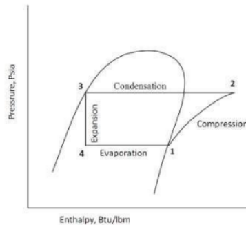
Figure 1. Vapor Compression Cycle of Refrigeration System
