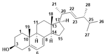
Figure 5. Structure of ergosta-5,7,22-trien-3 \beta -ol (ergosterol)
