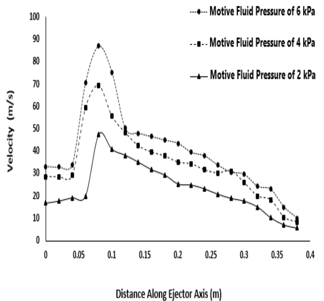
Figure 4. Flow velocity distribution along ejector axis
