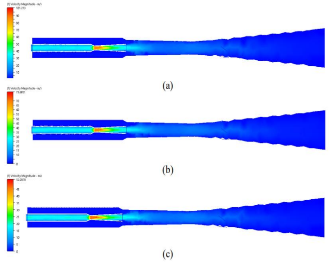
Figure 3. Flow velocity contours inside ejector: (a) 6 kPa, (b) 4 kPa, (c) 2 kPa
