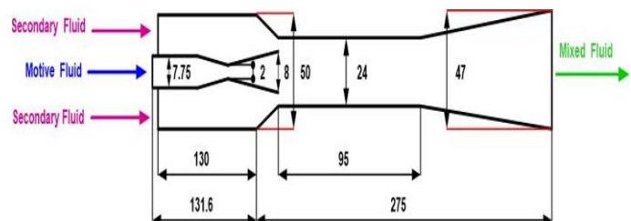
Figure 1. The construction and dimension of ejector
