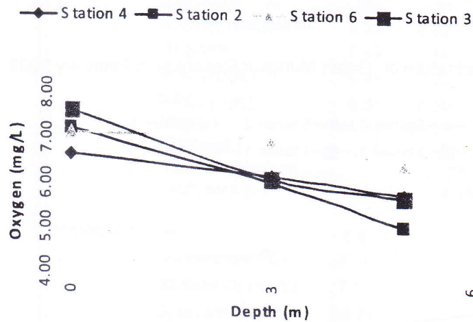
Figure 4. Dissolved oxygen of Gajah Mungkur Reservoir in February 2009.
