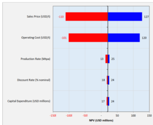
Gambar 9. Diagram Tornado – Sensitivitas
