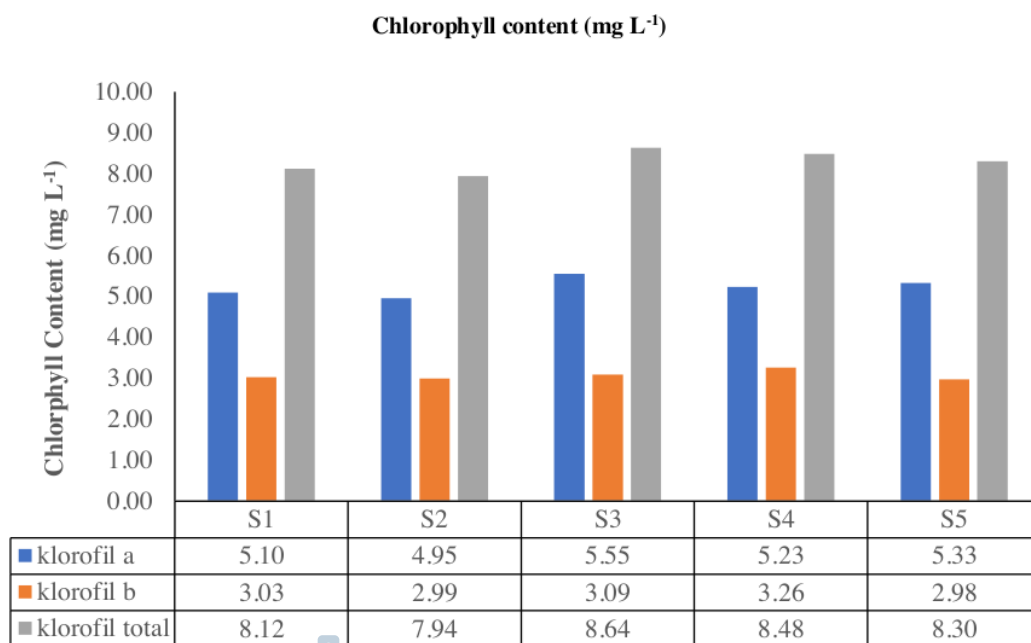
Figure 7. Average content of chlorophyll a, chlorophyll b and total chlorophyll.
