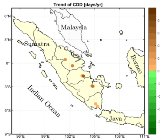
Figure 2. Spatial Distribution of CDD Trend in Selected Stations
