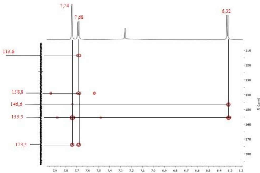
Figure 7. ^{13}\text{C} HMBC spectrum of 2,5-dihydroxyphenylethanone
