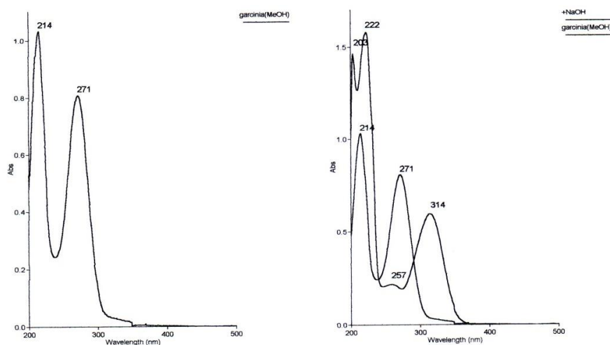
Figure 2. UV spectrum of 2,5-dihydroxyphenylethanone
