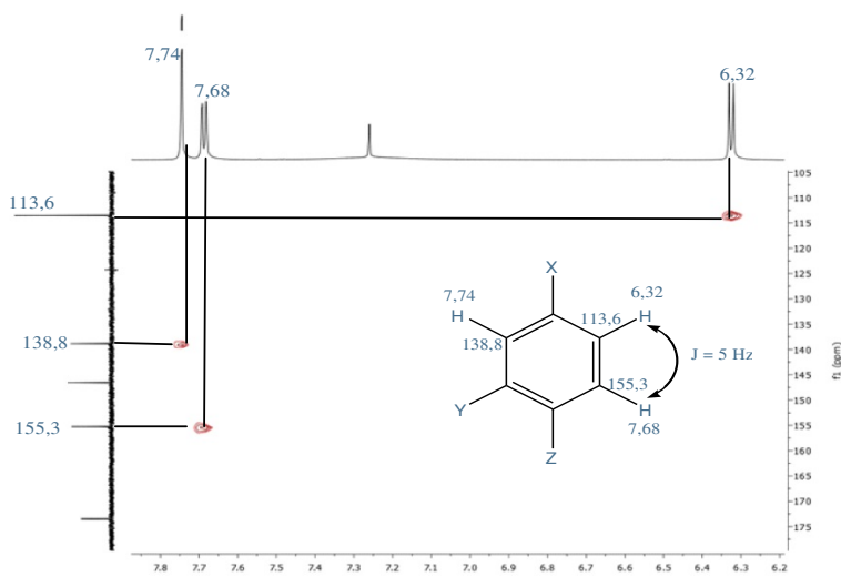
Figure 6. HMBC Spectrum of 2,5-dihydroxyphenylethanone
