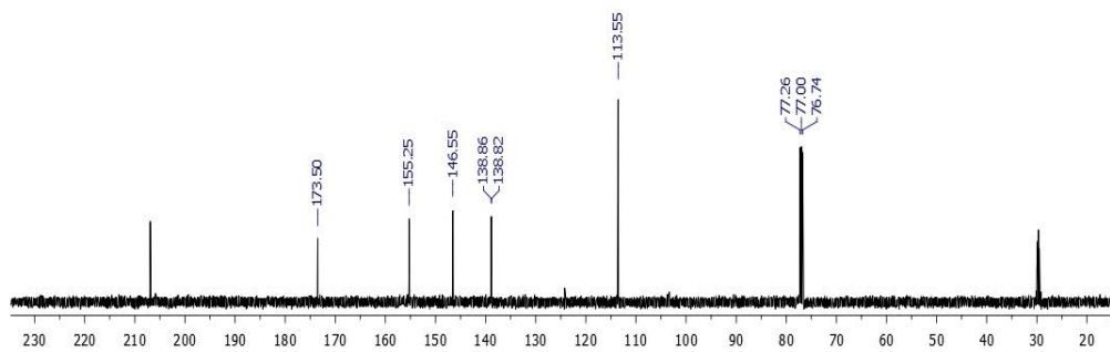
Figure 5. ^{13}\text{C} NMR spectrum of 2,5-dihydroxyphenylethanone
