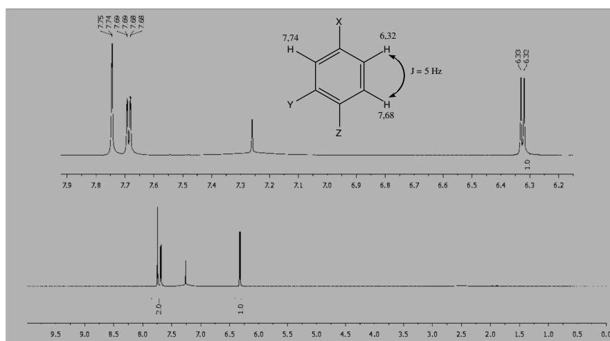
Figure 4. ^1\text{H} NMR spectrum of 2,5-dihydroxyphenylethanone
