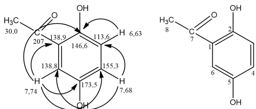
Figure 8. HMBC correlation and structure 2,5-dihydroxy-phenylethanone
