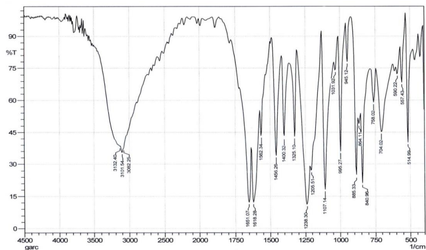
Figure 3. IR spectrum of 2,5-dihydroxyphenylethanone
