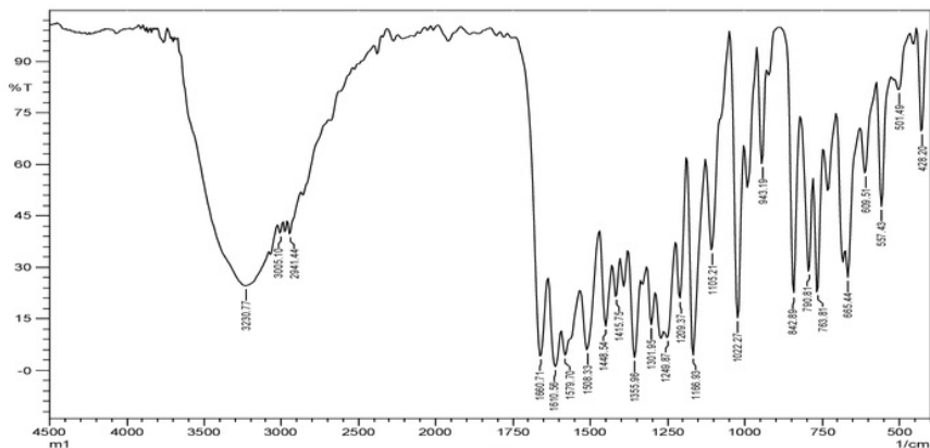
Figure 3. IR spectrum of isolated compound.
