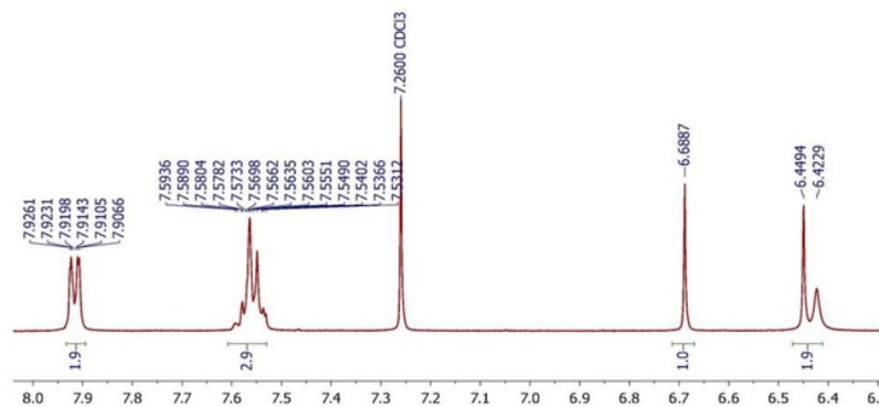
Figure 4. Spectra ^1\text{H} NMR of isolated compound
