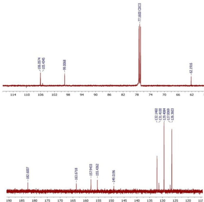
Figure 5. Spectrum ^{13}\text{C} NMR isolated compound.
