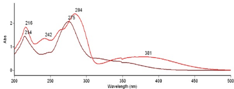
Figure 2. UV Spectrum of isolated compound.
