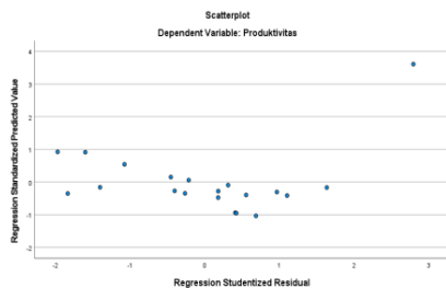
Figure 2. Scatterplot method heteroscedasticity test
