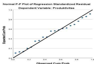
Figure 1. Normality test normal statistical method P-Plot test
