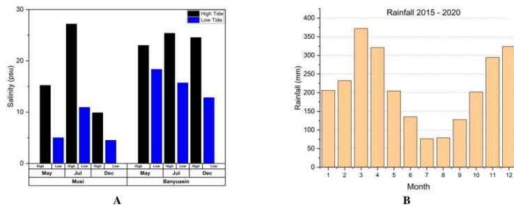
Figure 3. A. The average salinity in each data collection period, B. average rainfall for the period 2015 to 2020
