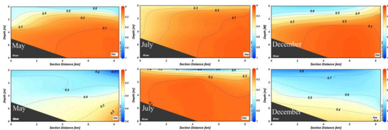
Figure 8. The cross-sectional profile of the freshwater fraction from the estuary to the sea in the Banyuasir River, South Sumatra, Indonesia in different seasons. Flood period ( top ) and ebb period ( bottom )
