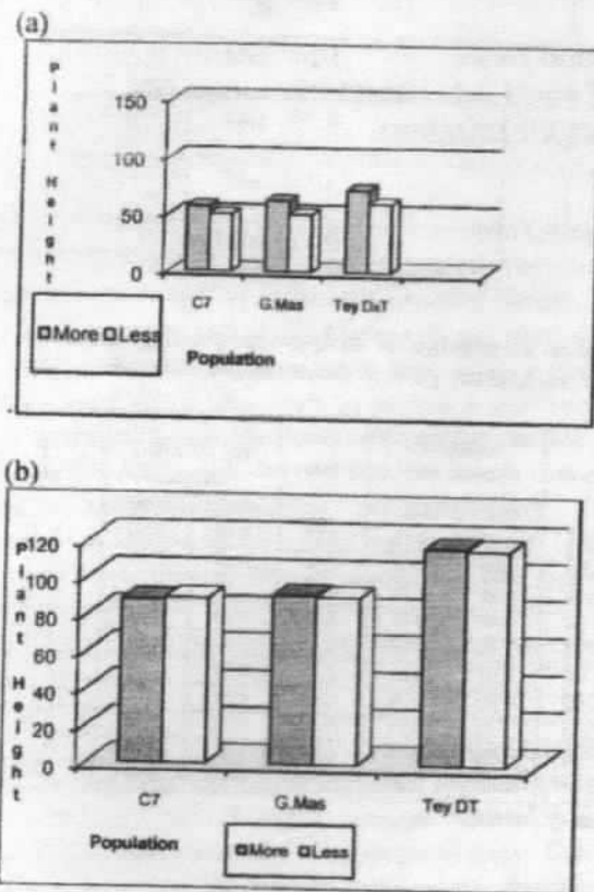
Figure 2. Plant height (cm) of more and less tolerant plants to aluminum measured at 15 (a) and 30 (b) days after planting on corn variety of C7, "Genjah Mas", and Tey DT
