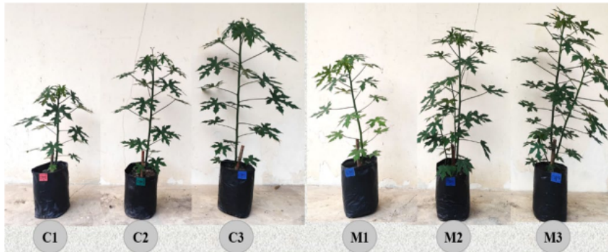
Figure 4. Performance of Chaya with various drought stress (A) and manure application (B).
