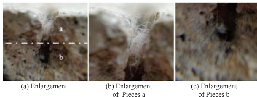
FIGURE 8. Detailed repair improvement on mortar
