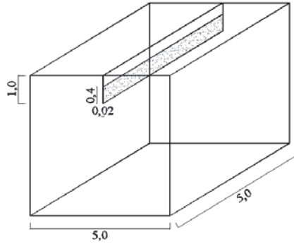
FIGURE 11. Mortar with a crack depth of 1 cm and a width of 0.2 mm
