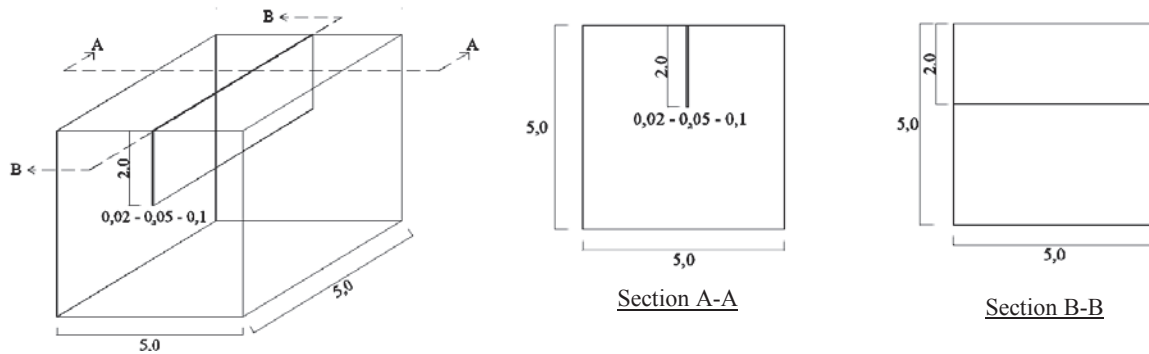
FIGURE 3. Artificial cracks in the test sample with 2 cm depth and 0.2, 0.5 and 1 mm width
