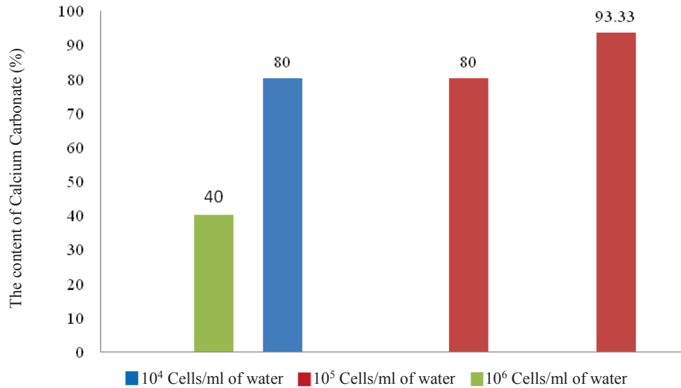
FIGURE 13. Graph of crack repair with 3 compositions
