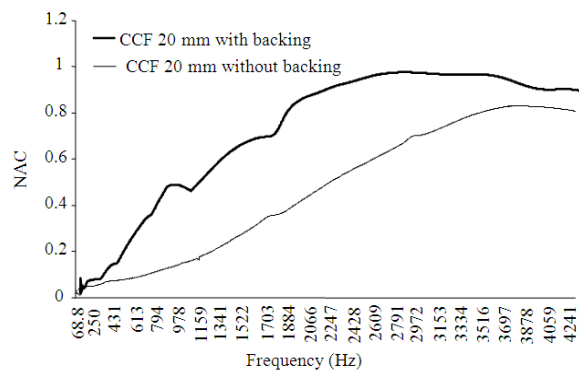
Fig. 6: Comparison of NAC versus CCF, 20 mm thickness, with and without porous layer backing
