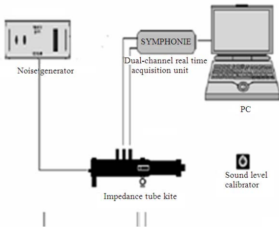
Fig. 2: Impedance tube device and set-ups for impedance tube measurement
