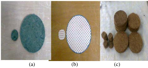
Fig. 1: Photographs of the test samples (a) porous layer; (b) perforated panel; (c) coconut coir fiber
