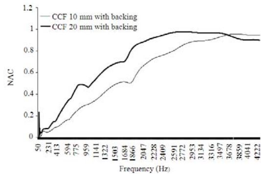
Fig. 4: The NAC of coconut coir fiber with porous layer backing
