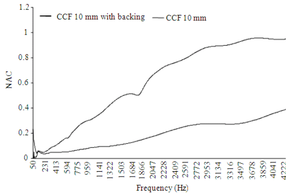
Fig. 5: Comparison of NAC of CCF, 10 mm thickness, with and without porous layer backing
