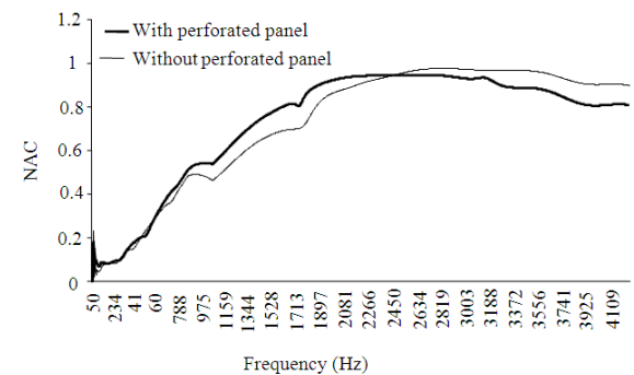
Fig. 7: Comparison of NAC of CCF, 20 mm thickness, with and without perforated panel backing
