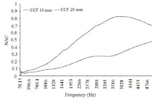
Fig. 3: The NAC coconut coir fiber without porous layer
