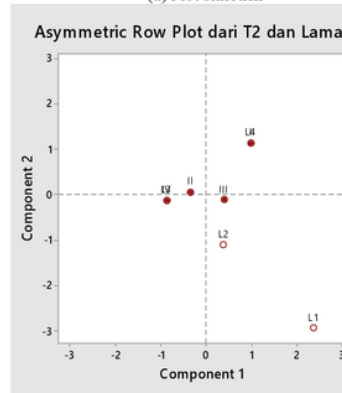
(b) Plot asimetrik
