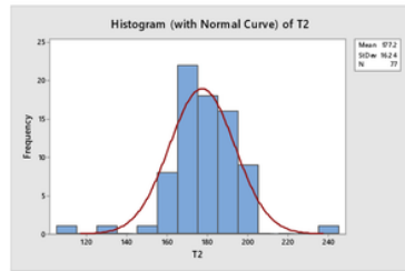
(c) Histogram T2
