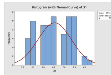
(a) Histogram X1
