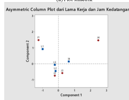
(b) Plot asimetrik
