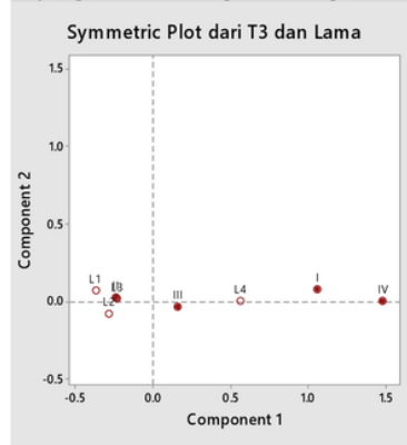
(a) Plot simetrik
