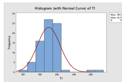
(b) Histogram T1
