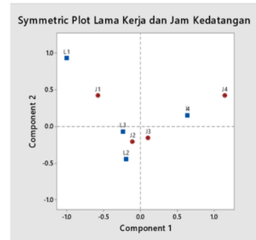
(a) Plot simetrik
