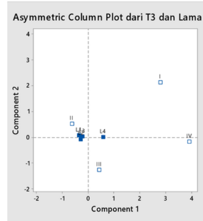
(c) Plot asimetrik
