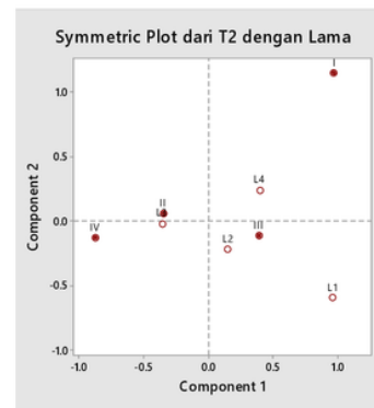
(a) Plot simetrik
