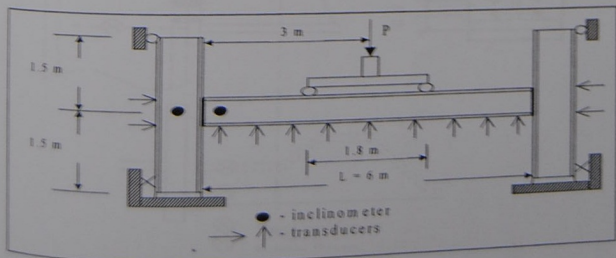
Figure 5: Locations of equipment for data acquisition
