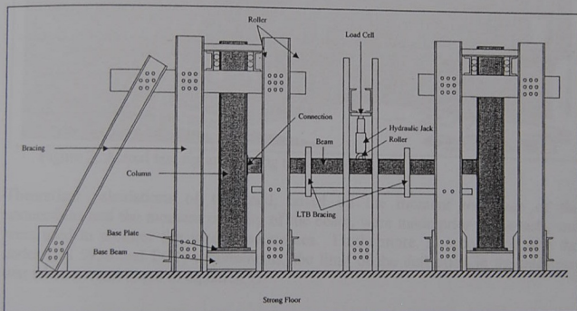
Figure 1: Testing arrangement
