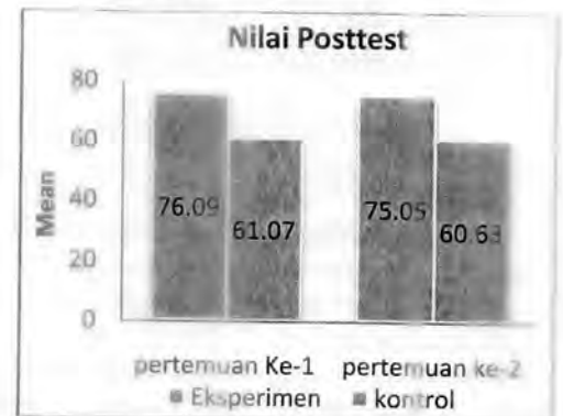
Gambar 5. Diagram Nilai Posttest Siswa
