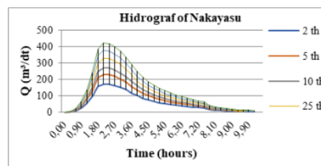
Fig. 9: Nakayasu Synthetic Hydrograph Lebak Semendawai irrigation
