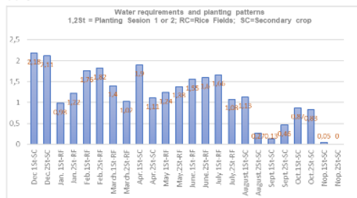
Fig.15: Irrigation Water Needs and Planting Pattern Plans
