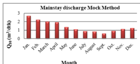
Fig. 8: Mainstay Discharge Method F.J. Mock
