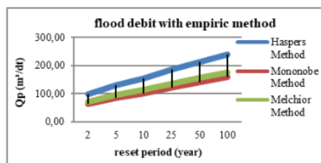
Fig. 11 : Flood Hydrograph of the Empirical Method Plan
