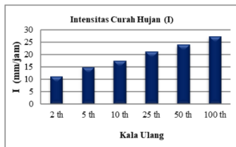
Fig. 7: Intensity of rainfall Mononobe method
