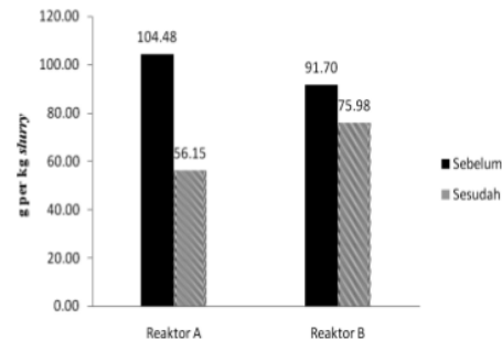
Gambar 6. Nilai Volatile Solids (VS)
