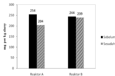
Gambar 3. Nilai Biochemical Oxygen Demand (BOD)
