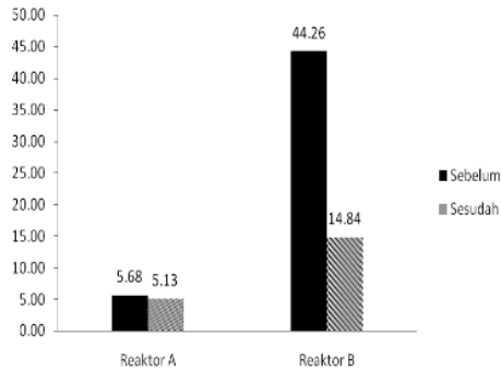
Gambar 7. Nilai rasio C/N slurry.
