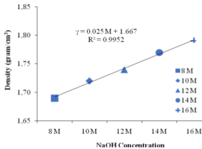
Fig. 9. Density vs NaOH concentration in 28 th day.
