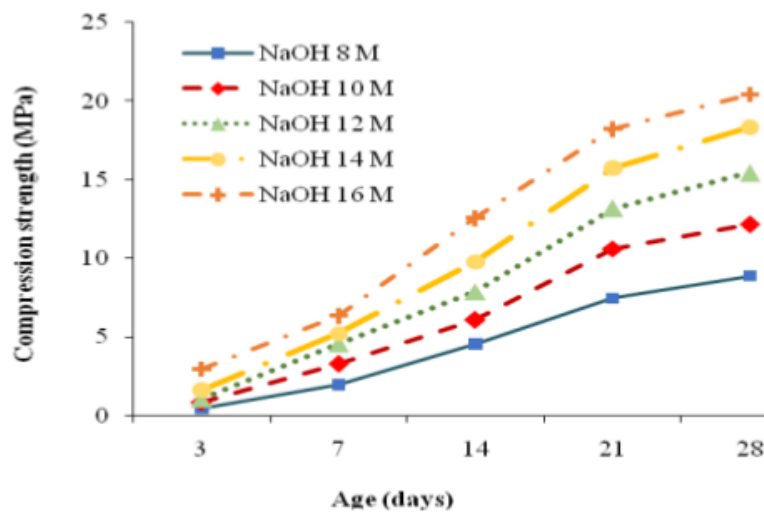
Fig. 6. Compressive strength.
