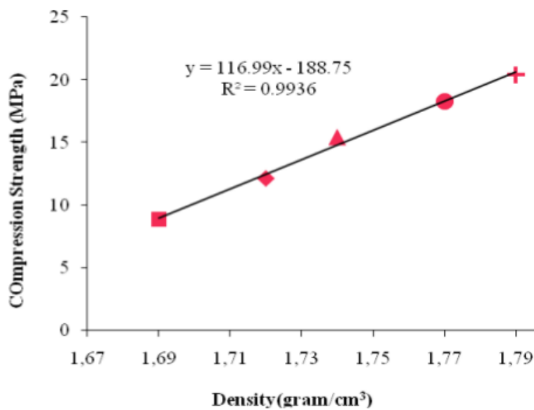
Fig. 7. Compressive strength vs density in 28 th day.
