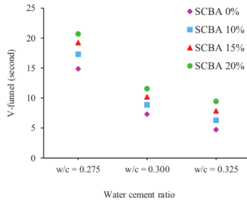
FIGURE 8. The effect of w/c variation on V-funnel
