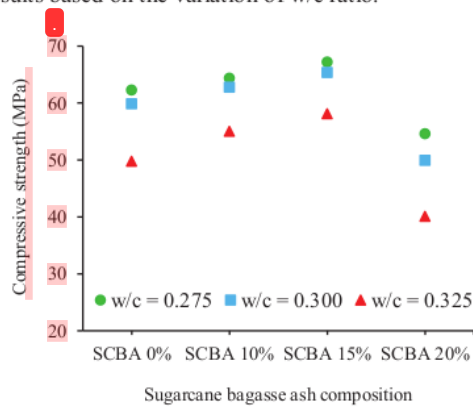
FIGURE 11. The effect of sugarcane bagasse ash composition on concrete compressive strength on age 28 days
