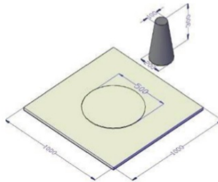
FIGURE 2. Slump flow test
