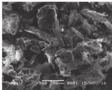
FIGURE 1. SEM test result of SCBA
