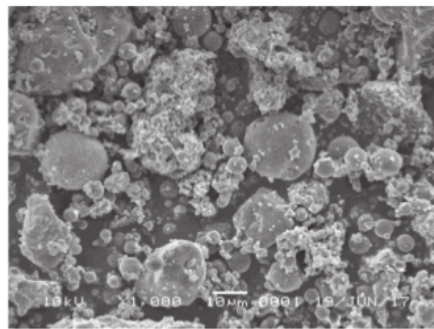
FIGURE 1. SEM microstructure fly ash
