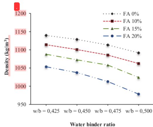
FIGURE 6. The effect of w/b variation on density at 28 days
