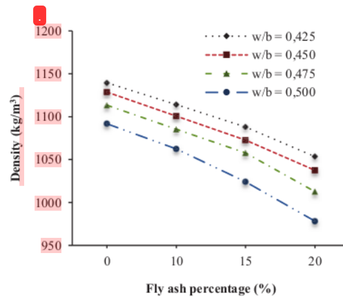
FIGURE 7. The effect of fly ash percentage on density at 28 days
