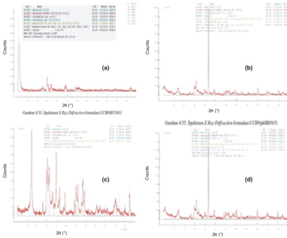
Fig. 3. (a) Spectrum XRD formula CCBNBT5651, (b) Spectrum XRD formula CCBNBPBB5651, (c) Spectrum XRD formula CCBNBPkCs5651, (d) spectrum XRD Formula CCBNBPkCs5651
