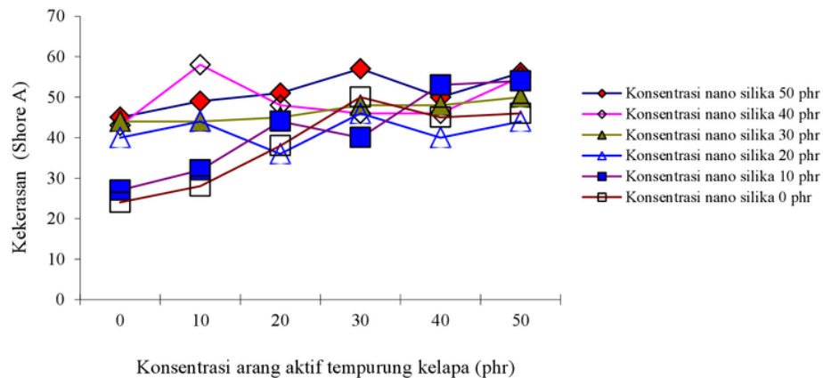
Gambar 1. Kekerasan komponen karet (Shore A)
